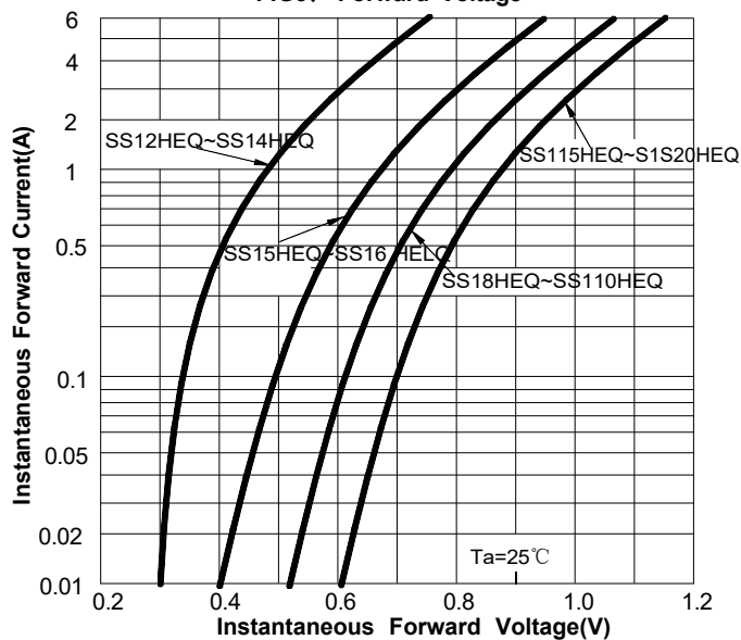
FIG3: Forward Voltage
