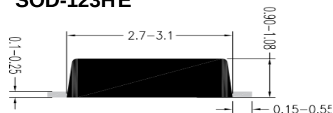
SOD-123HE
